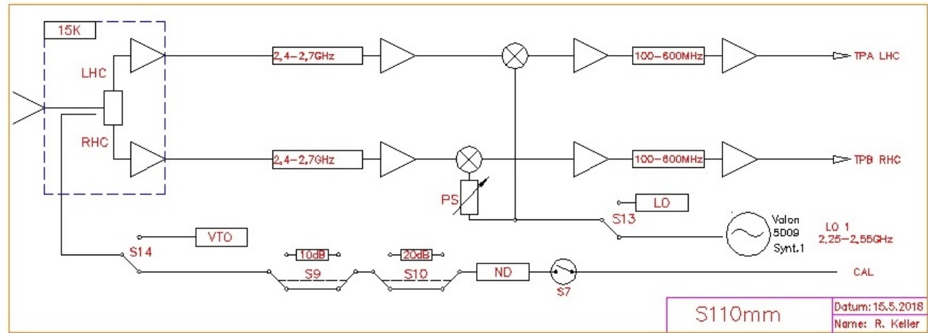
Simplified Block Diagram of the receiver, (RK on 15.5.2018)
