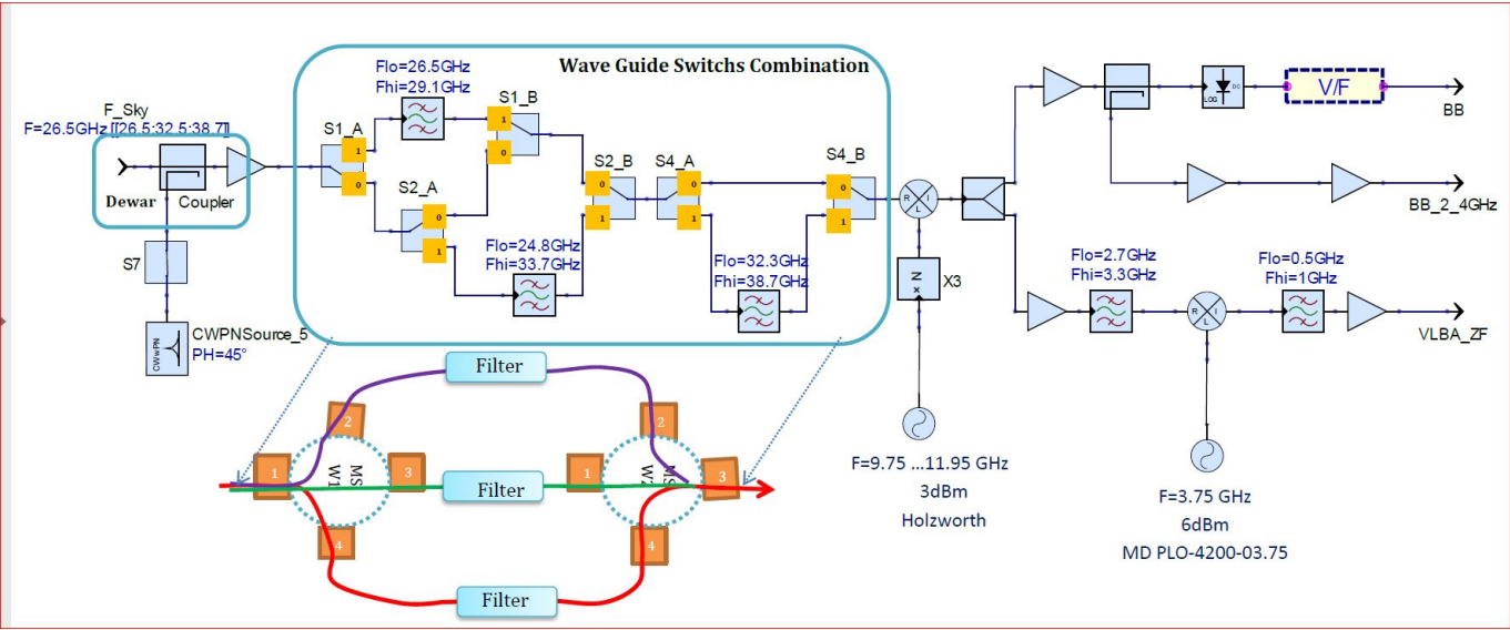
Simplified Block Diagram of p10mm_receiver_withholzworth.pdf , (ZMK on 26.03.2021)
