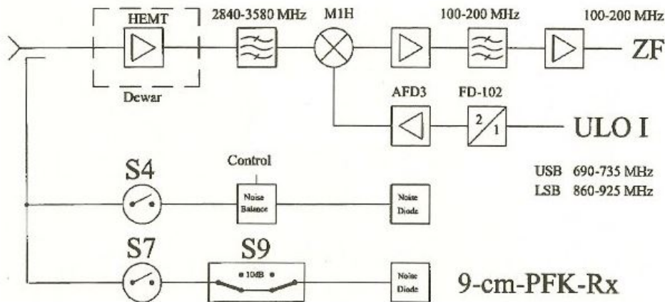
Block Diagram
