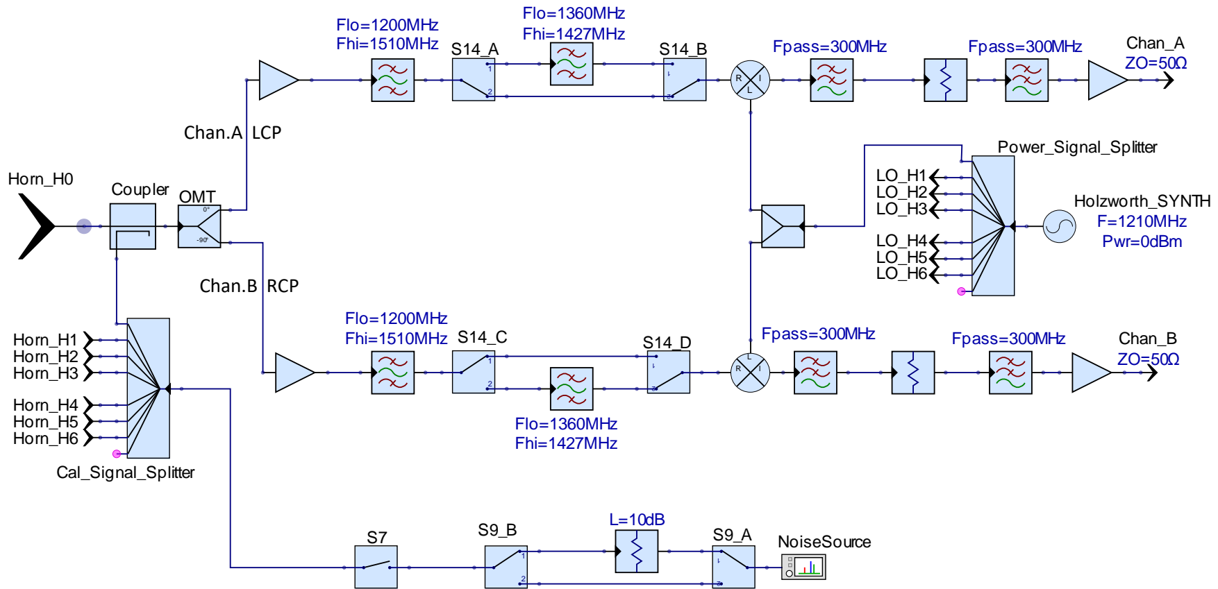
P127MM-7 Beam Receiver Block Diagram: One of the seven horns is shown in the diagram
