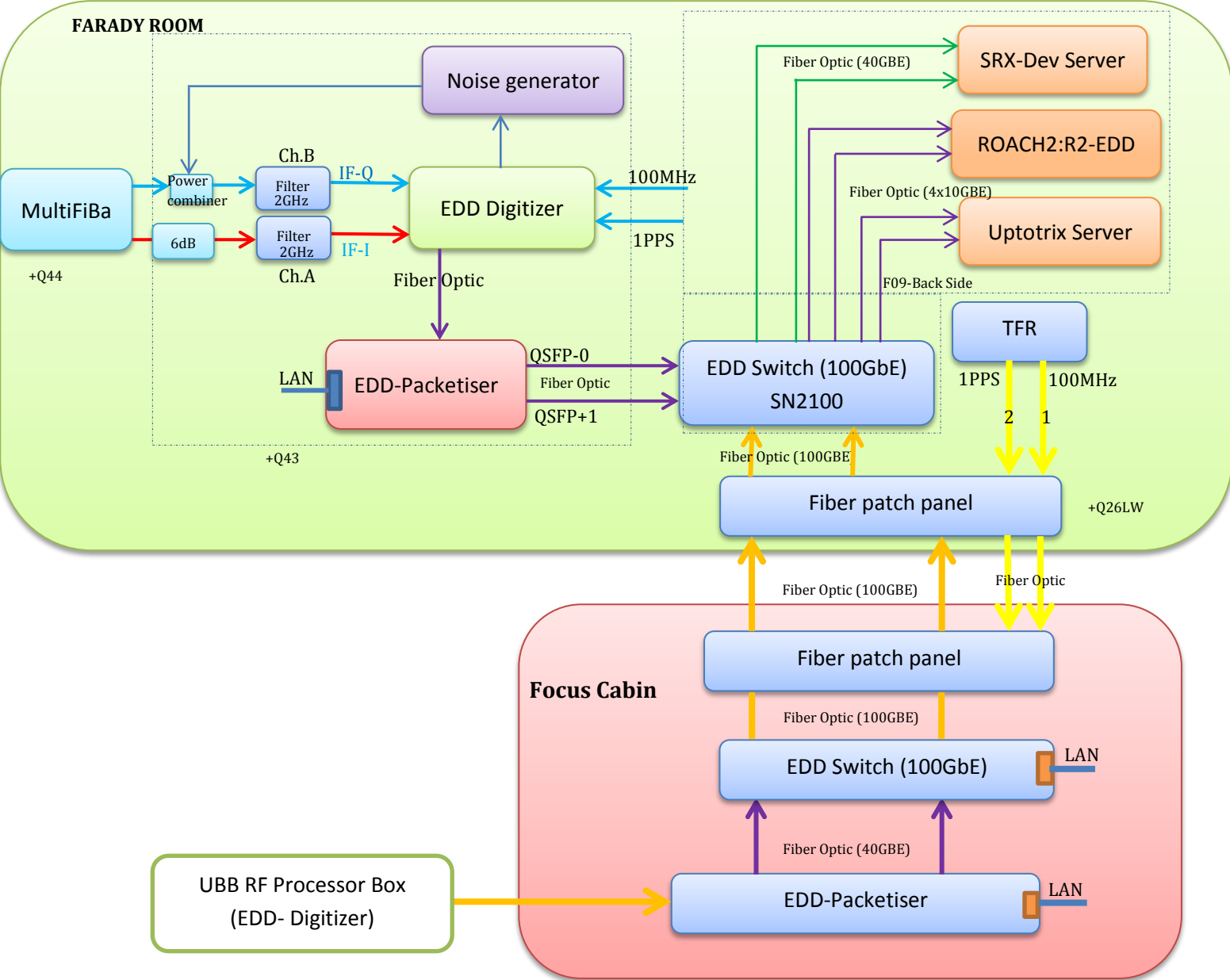
Currently deployed EDD Instrumentation and Signal Flow Diagram
