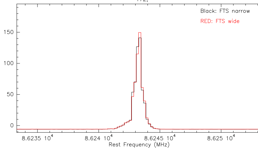
Figure 12: Comparing wide and narrow mode of the FTS. The narrow spectra has been smoothed to 200 kHz resolution to match the one of the wide mode.
