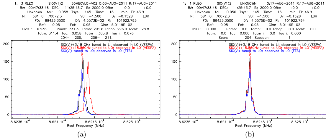
Figure 5: Plots of setups 2 through 4. All are observed in the LO. Black shows setup 2 tuning SiO(VI)+3.18 to LI; Red SiO(VI)+18.86 GHz tuned to UO and Blue SiO(VI) tuned to LO. Note in all setups the Local Oscillator frequency is the same and it was not retuned. a) The shift gets larger if the distance to the specified sub-band is larger. b) Re-Reduced spectra as in Figures 1 and 3.
