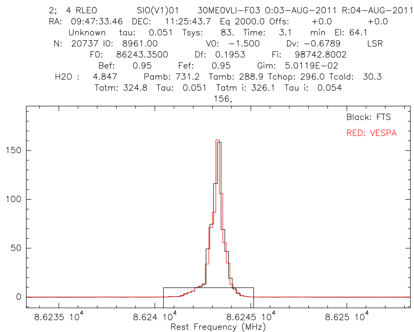
Figure 9: Comparing Vespa spectra smoothed to \sim 200 kHz resolution with the corresponding wide FTS spectra. Flux and Position are consistent.
